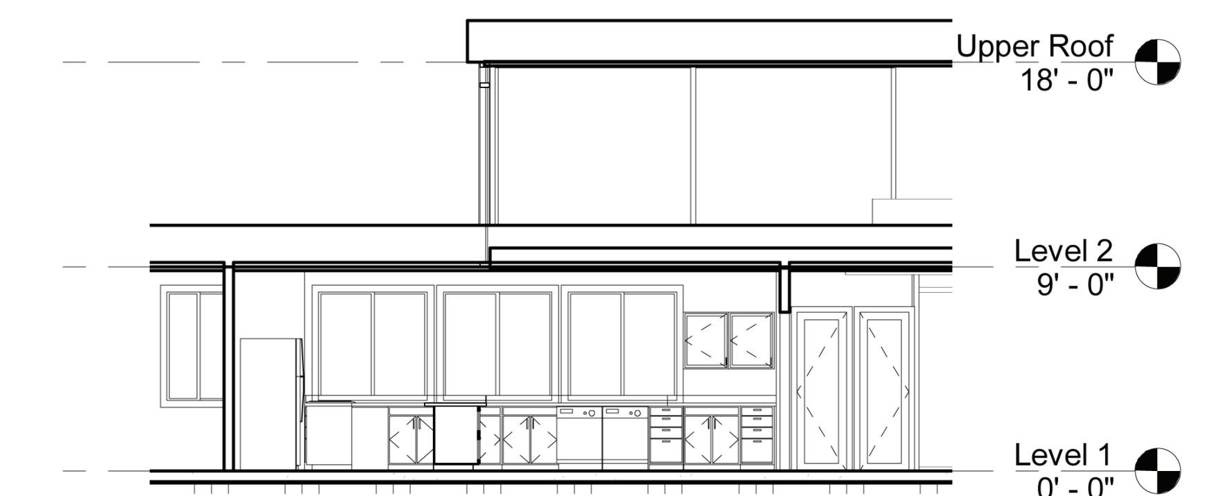
Kitchen Detail Elevation
