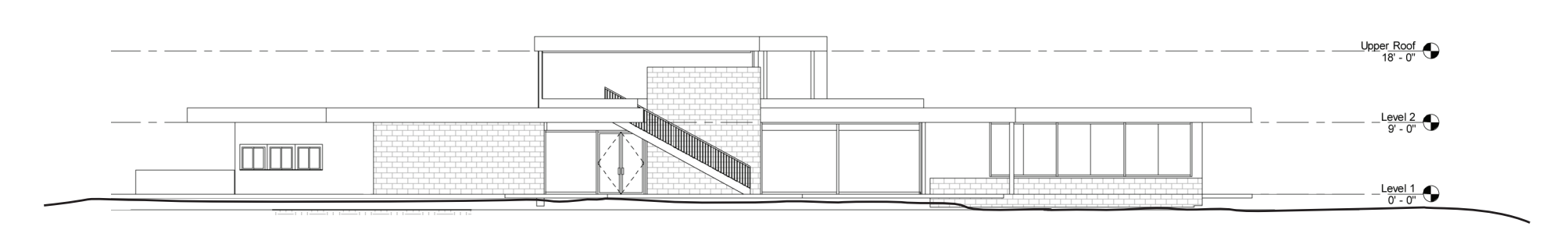
South Elevation
