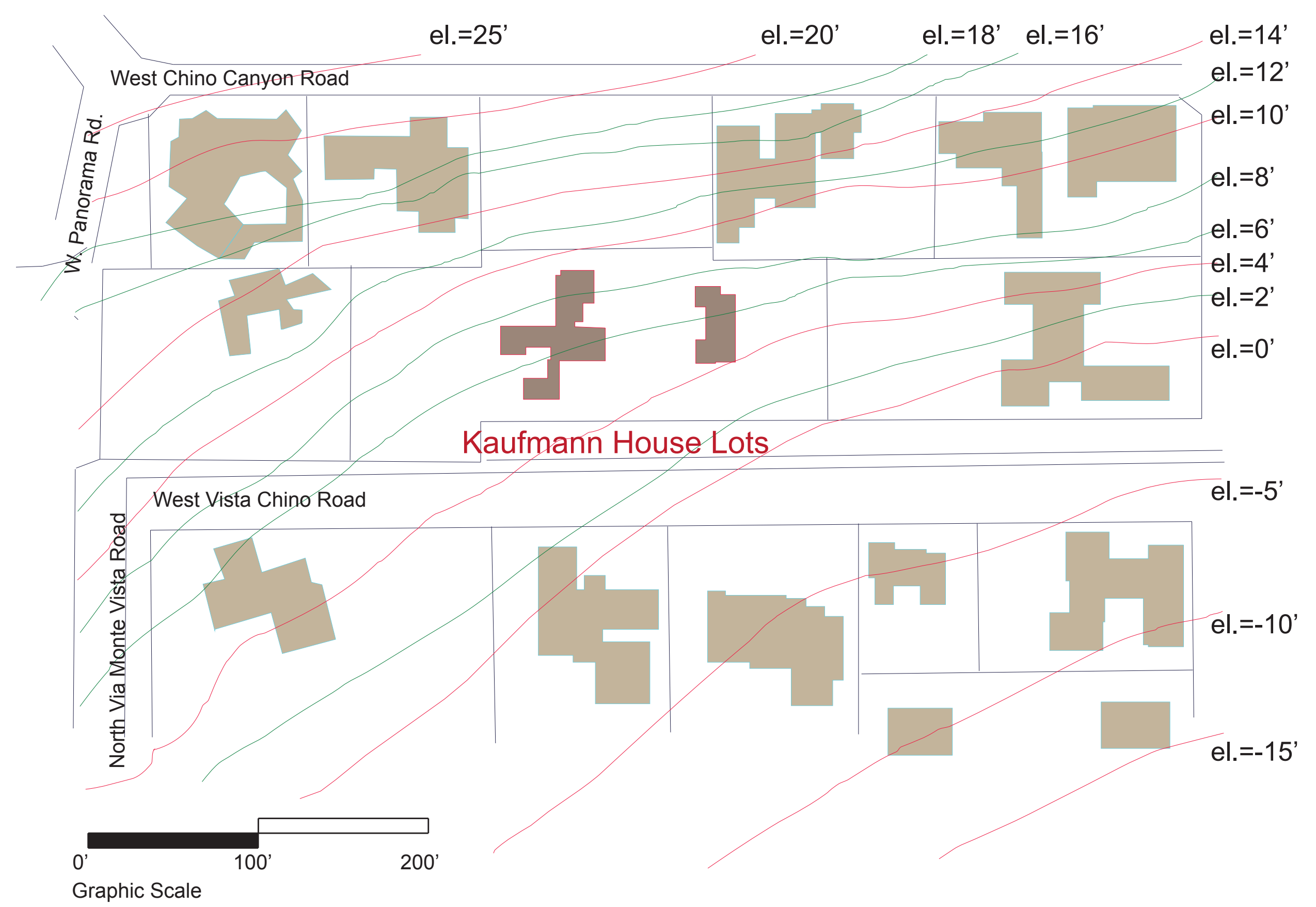
Kaufmann House Site plan and local context
